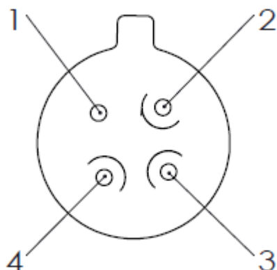
Figure 1 Bottom View
