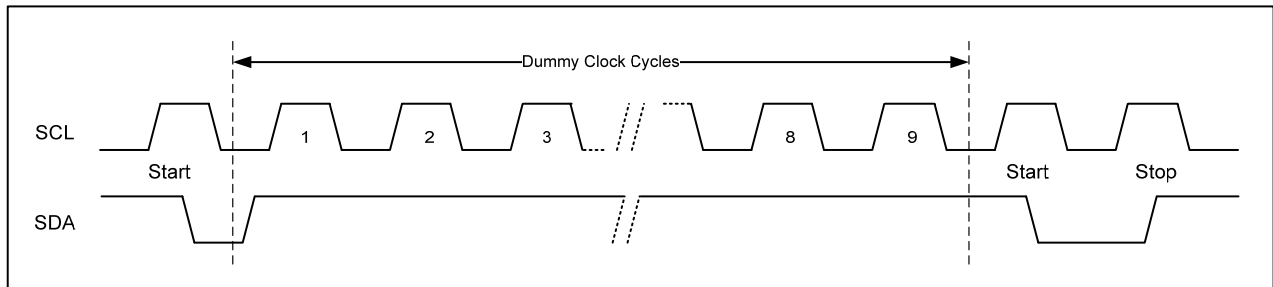
Figure4 Soft Reset
