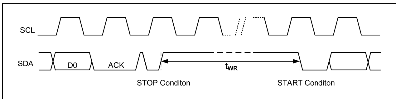
Figure12 Bus Timing
