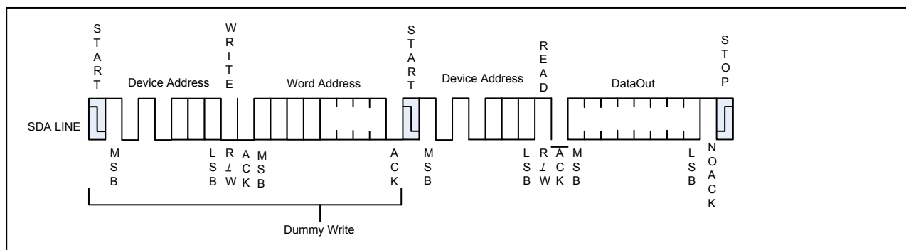
Figure8 Random Read
