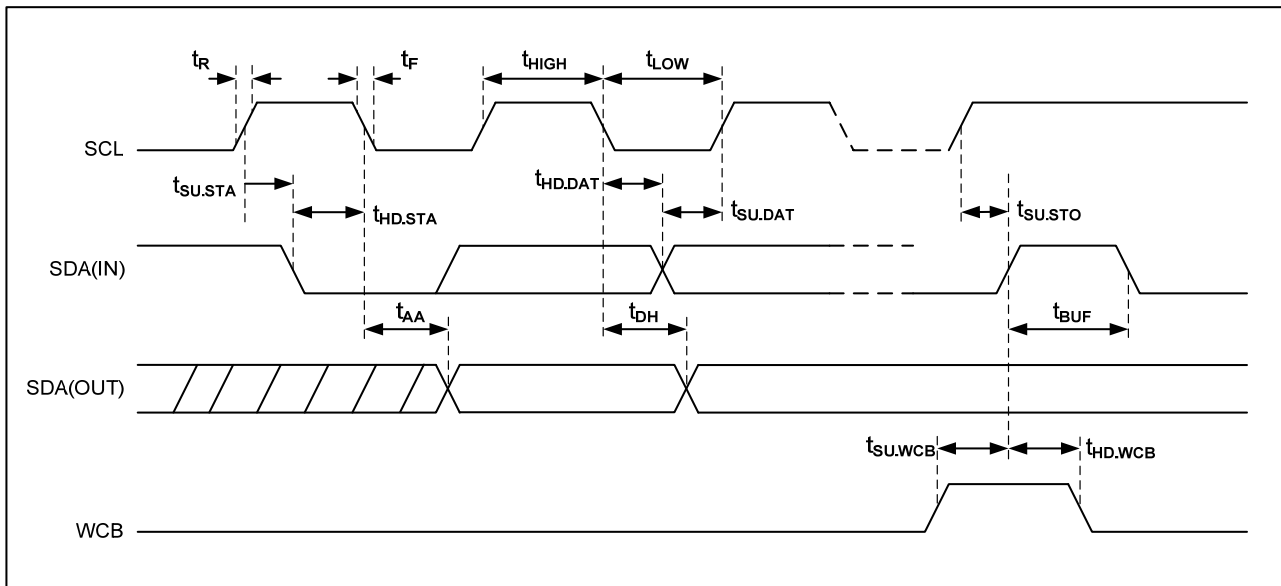
Figure10 Bus Timing
