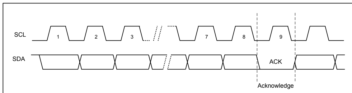
Figure3Output Acknowledge
