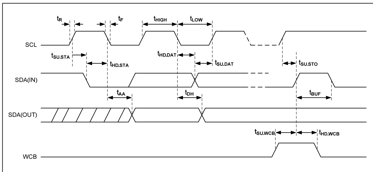
Figure12 Bus Timing
