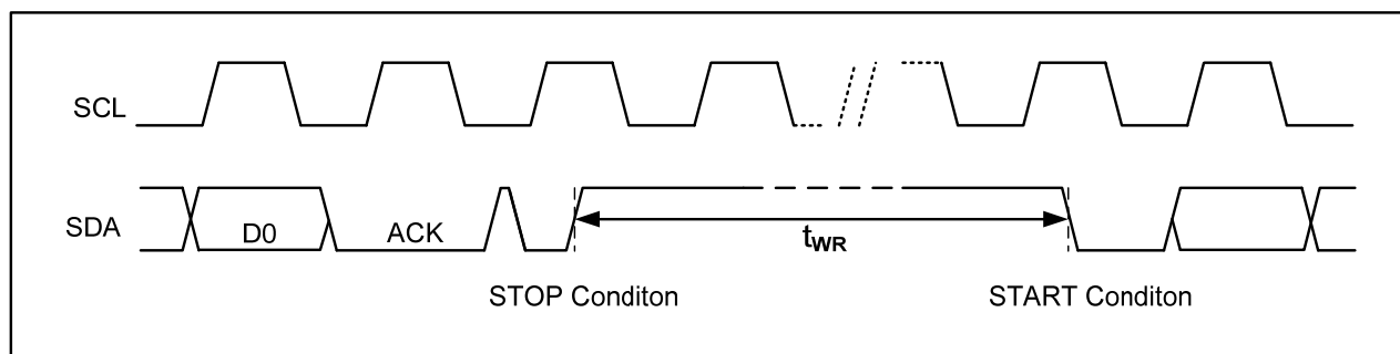
Figure12 Bus Timing
