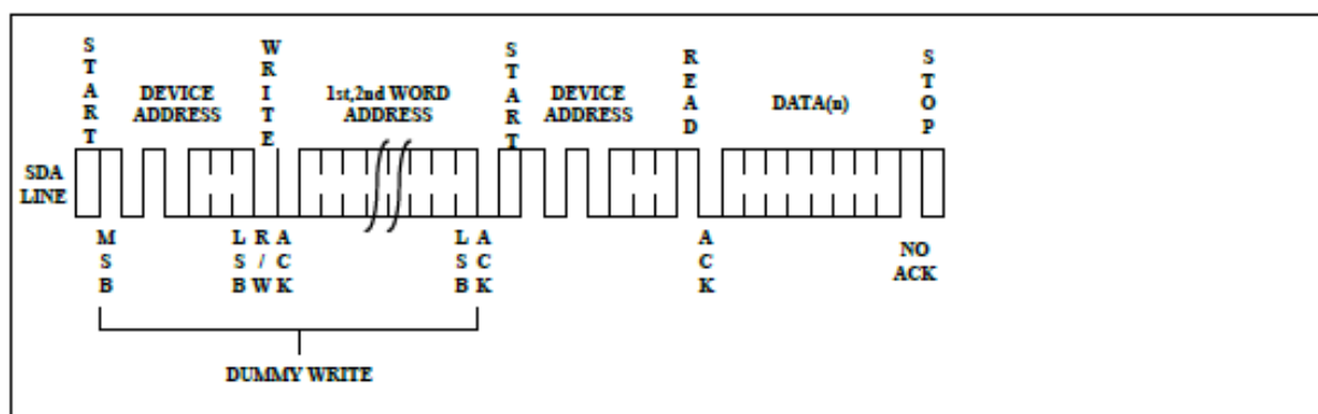
Figure7 Random Read
