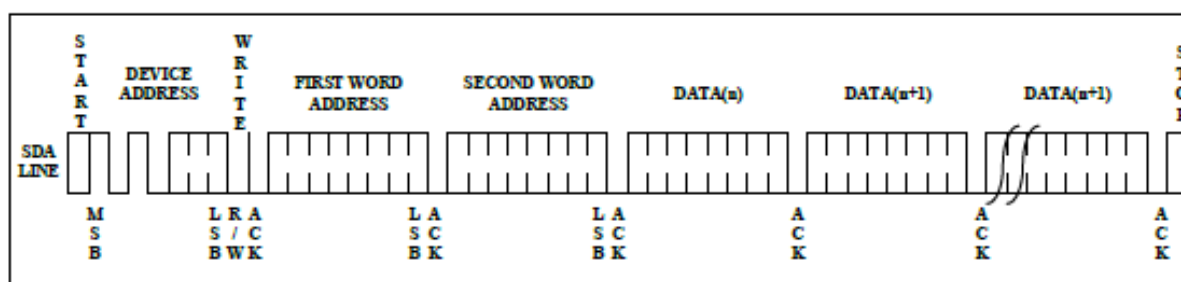
Figure5 Page Write
