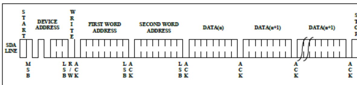
Figure5 Page Write
