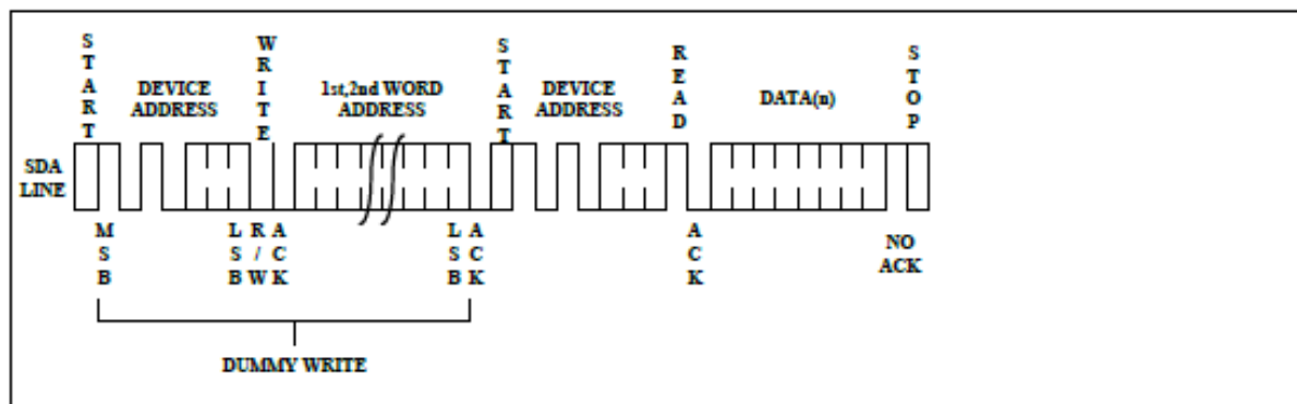
Figure7 Random Read
