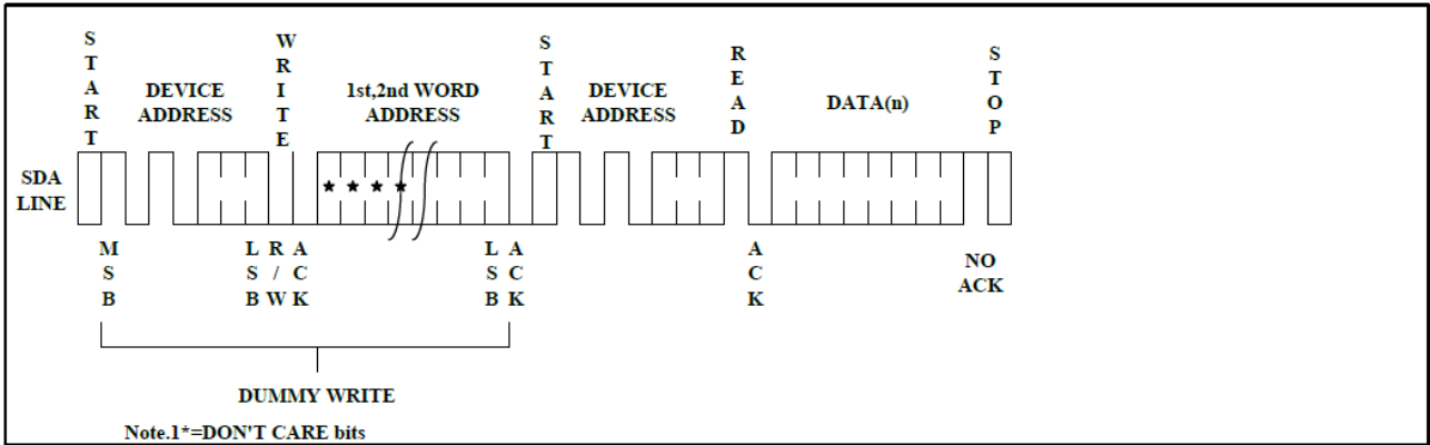
Figure7 Random Read
