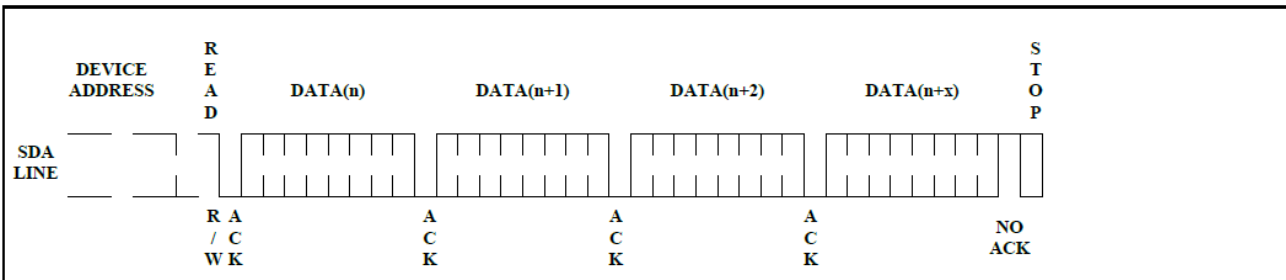
Figure8 Sequential Read
