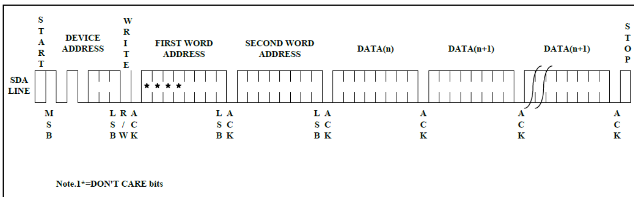
Figure5 Page Write
