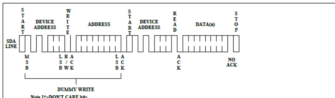
Figure7 Random Read
