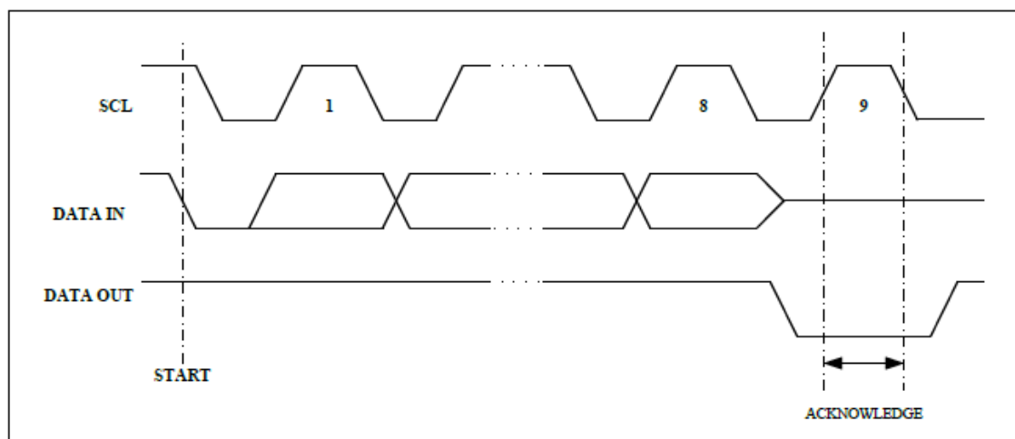
Figure3 Output Acknowledge
