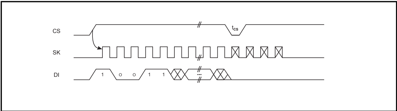
Figure 3. EWEN Timing
