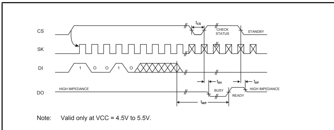
Figure 8. ERAL Timing
