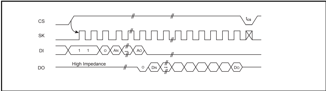
Figure 2. READ Timing
