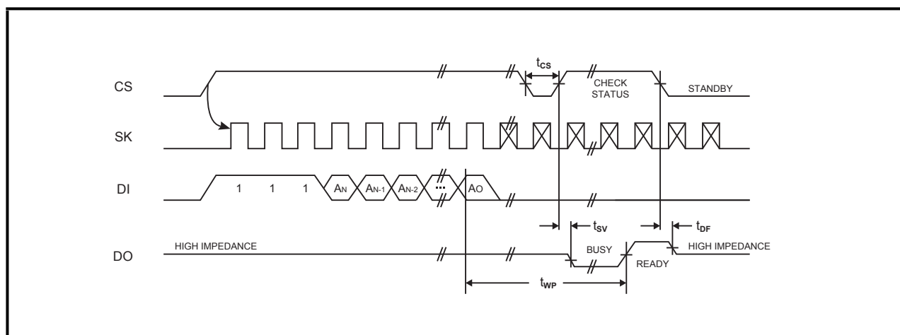
Figure 7. ERASE Timing
