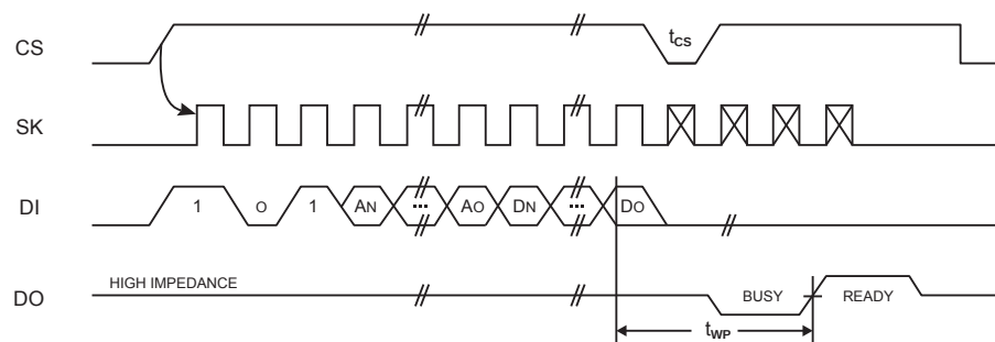
Figure 6. WRAL Timing
