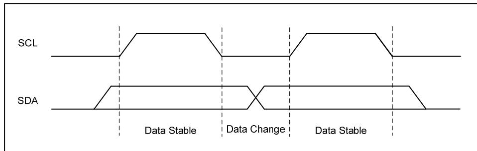
Figure4 Data Validity
