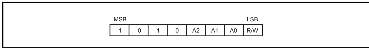
Figure8 Device Address
