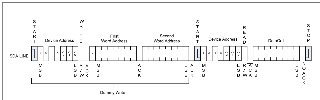
Figure12 Random Read
