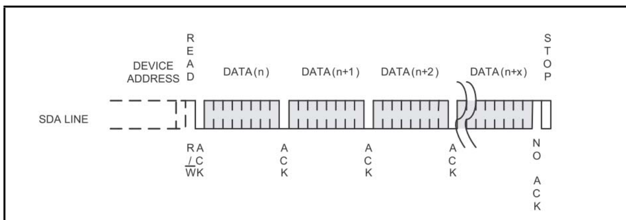
Figure 9. Sequential Read
